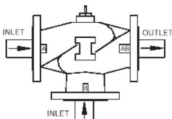
Valvola a 3 vie miscelatrice
