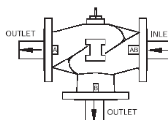
Valvola a 3 vie deviatrice
